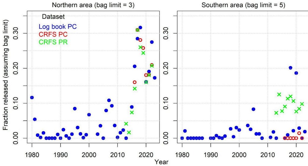
Figure 3.1. Empirical evaluation of theoretical release fraction given the specified bag limits only for halibut (given the observed catch rates per trip, what fraction would have been released if the bag limit were adhered to perfectly).
