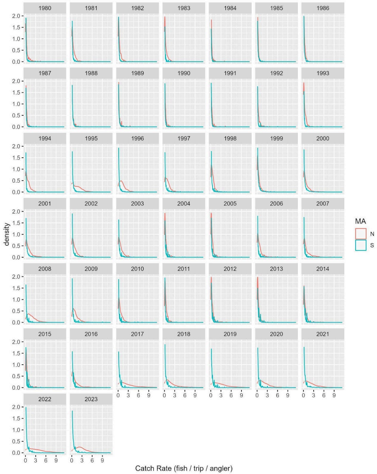
App. Figure. 1. Log book party charter catch rate distributions by year for the northern (N) and southern management areas (S).
